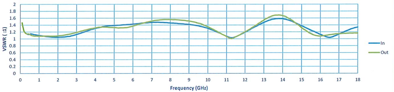
VSWR @ -20 dB
