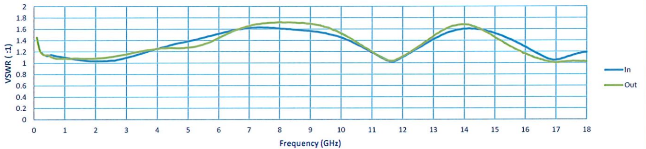
VSWR @ -20 dB
