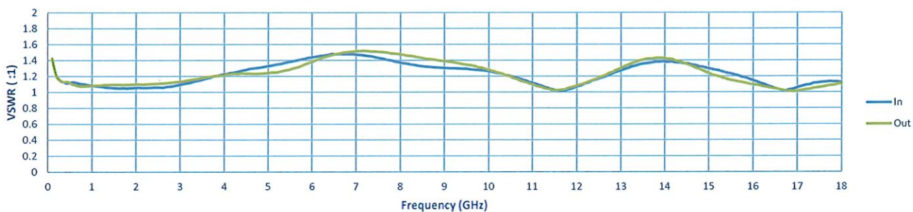
VSWR @ -20 dB
