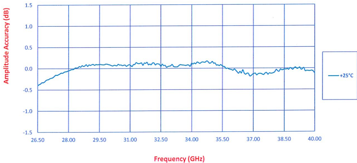
Amplitude Accuracy Vs Frequency
