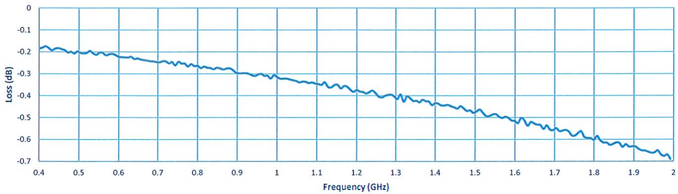
Insertion Loss
