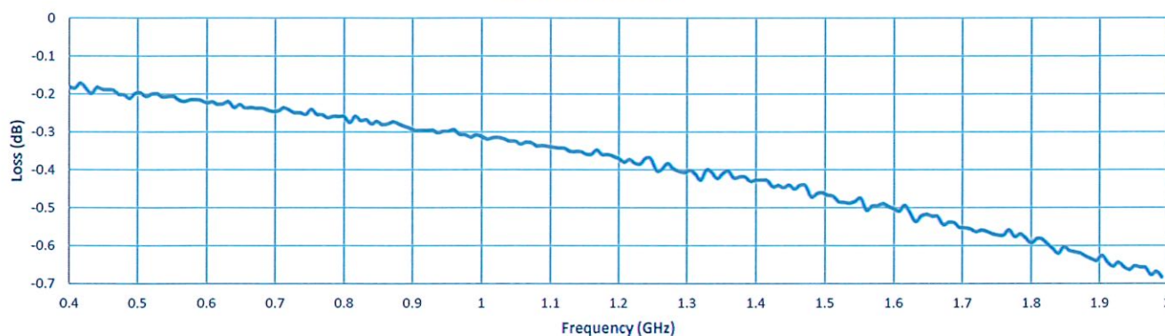
Insertion Loss
