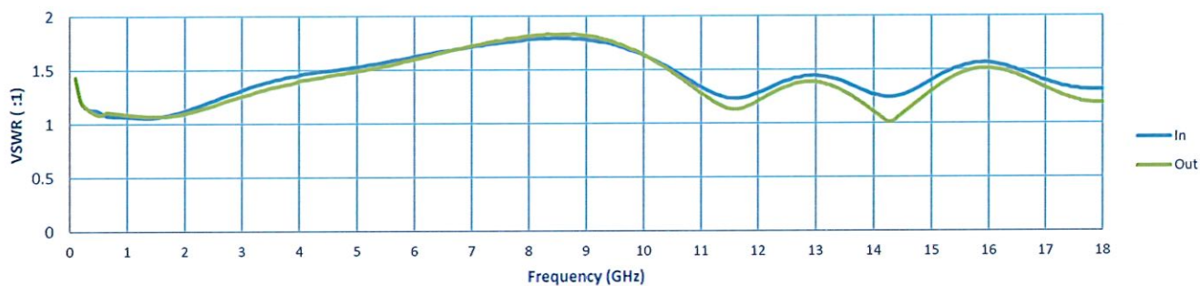
VSWR @ -20 dBm
