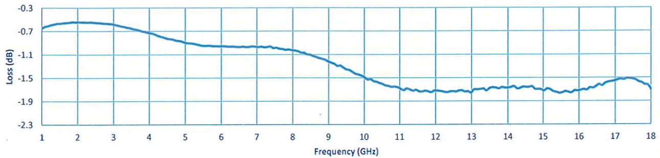
Insertion Loss
