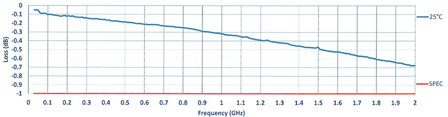
Insertion Loss
