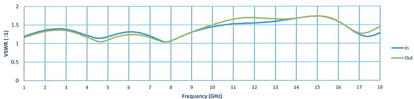
VSWR @ -20 dBm
