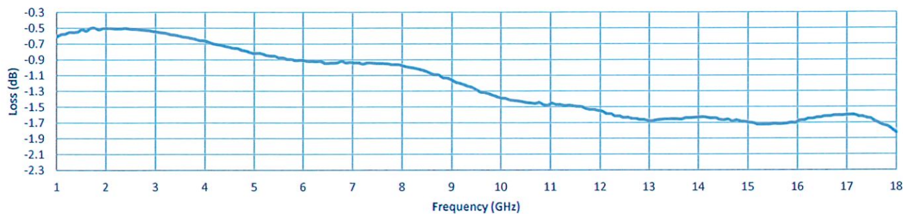
Insertion Loss
