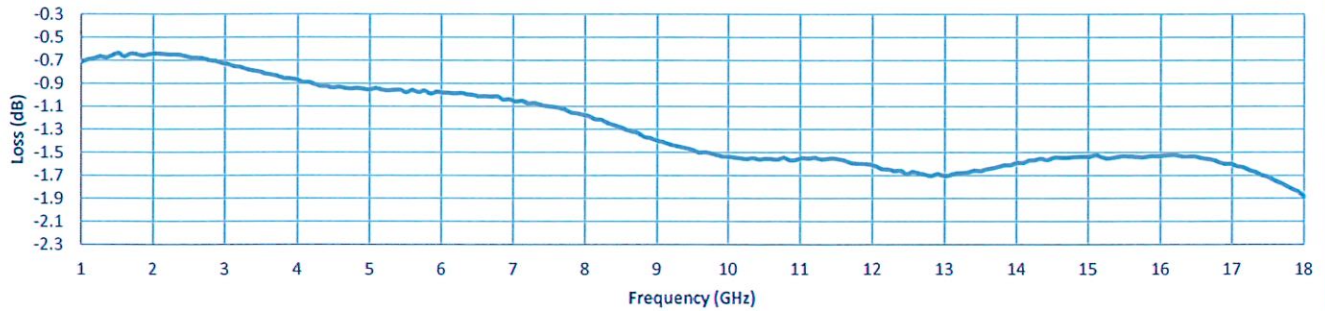
Insertion Loss
