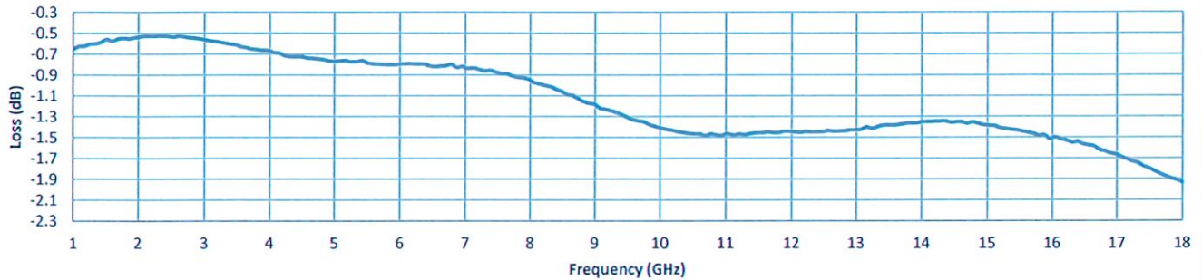
Insertion Loss
