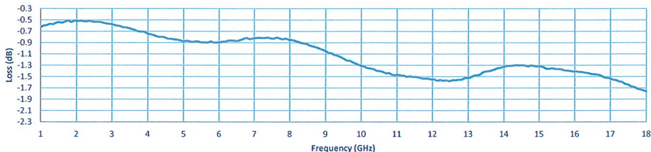
Insertion Loss
