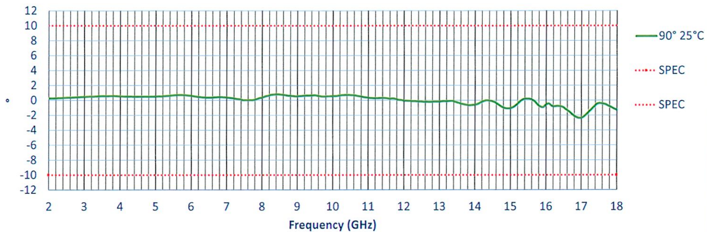
Phase Balance
