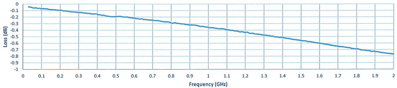
Insertion Loss @ 0dBm
