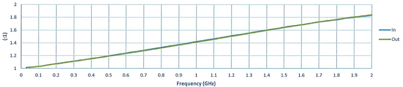
VSWR @ 0 dBm
