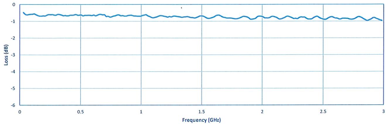
Insertion Loss
