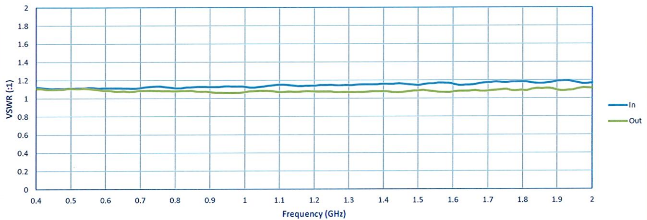
Limiter Response with Frequency
