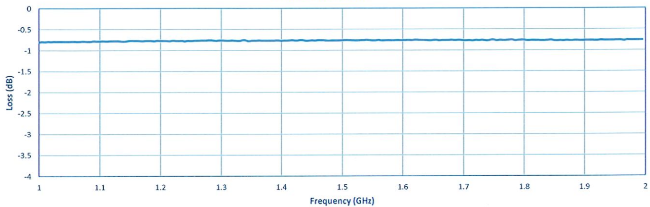
Insertion Loss
