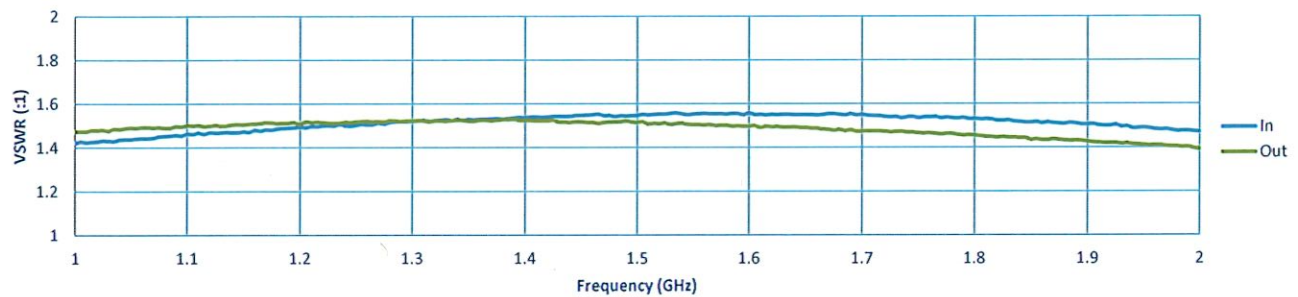
VSWR @ -10 dBm
