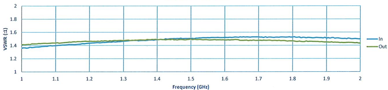
VSWR @ -10 dBm
