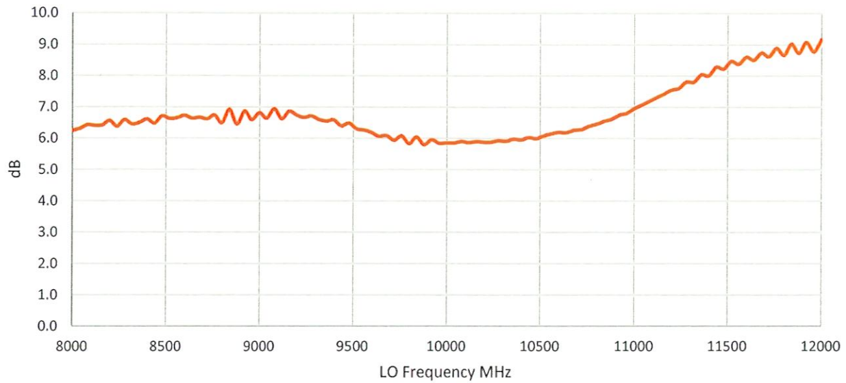
Conversion Loss
