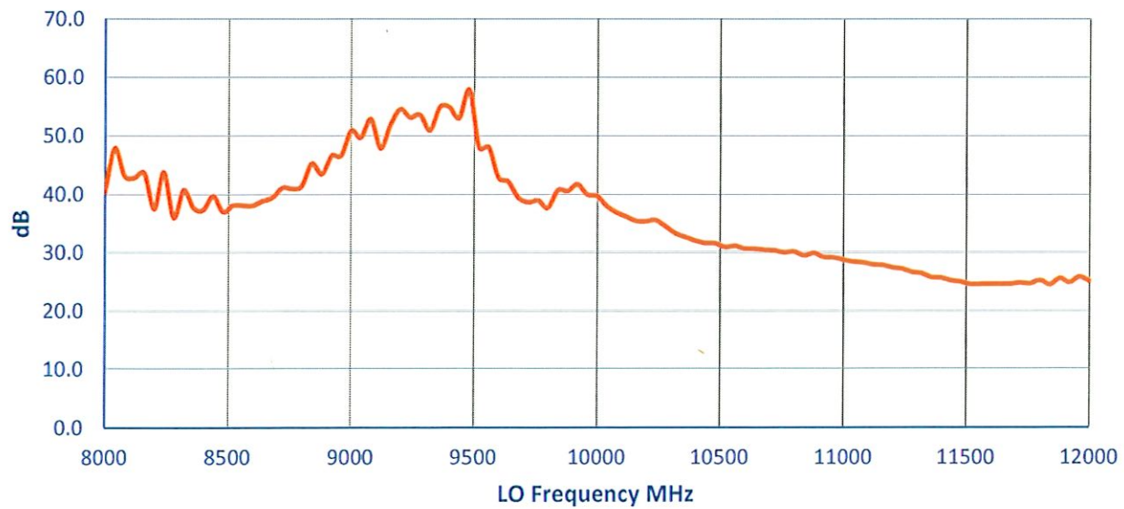
Image Rejection
