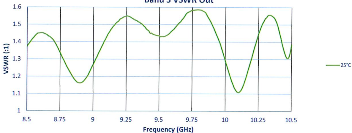
Band 3 VSWR Out
