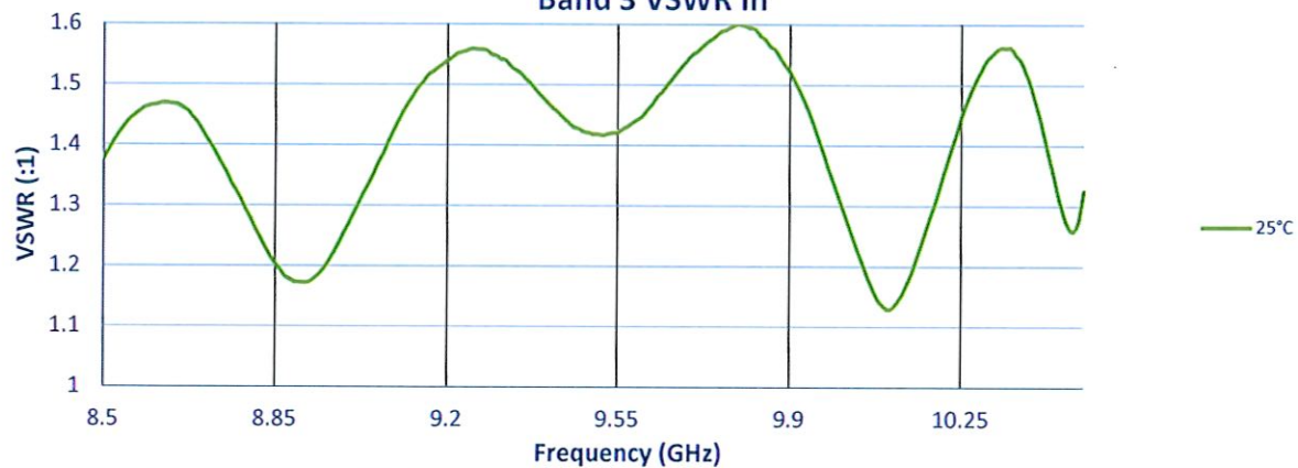
Band 3 VSWR In
