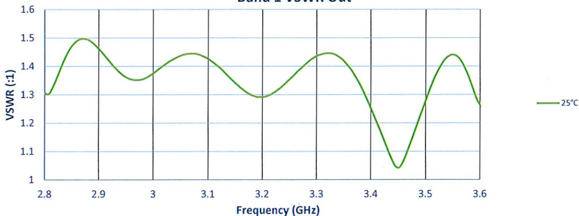
Band 1 VSWR Out
