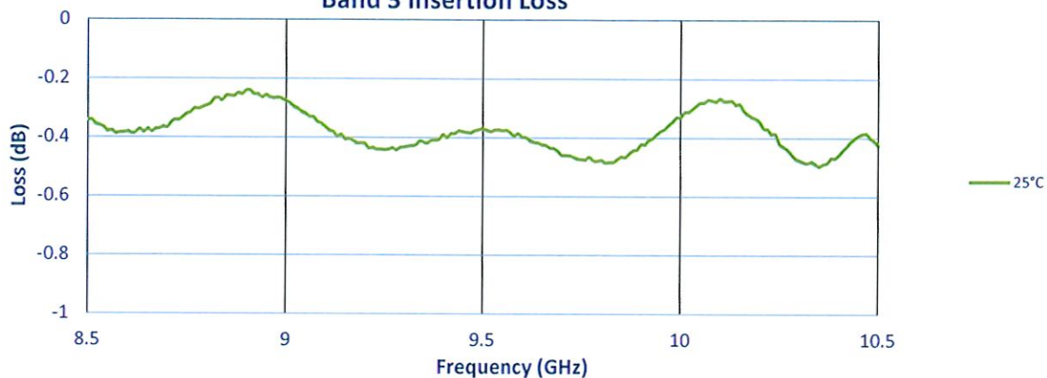
Band 3 Insertion Loss
