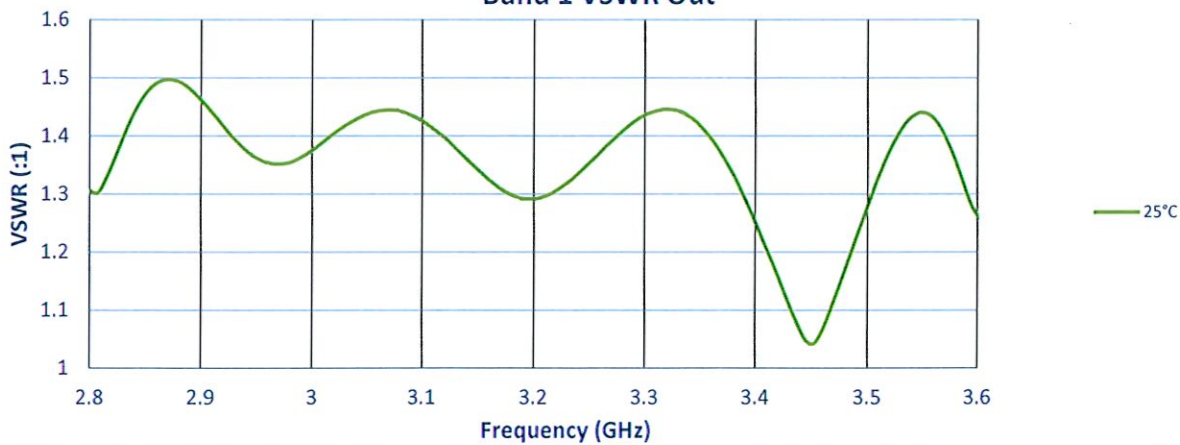
Band 1 VSWR Out
