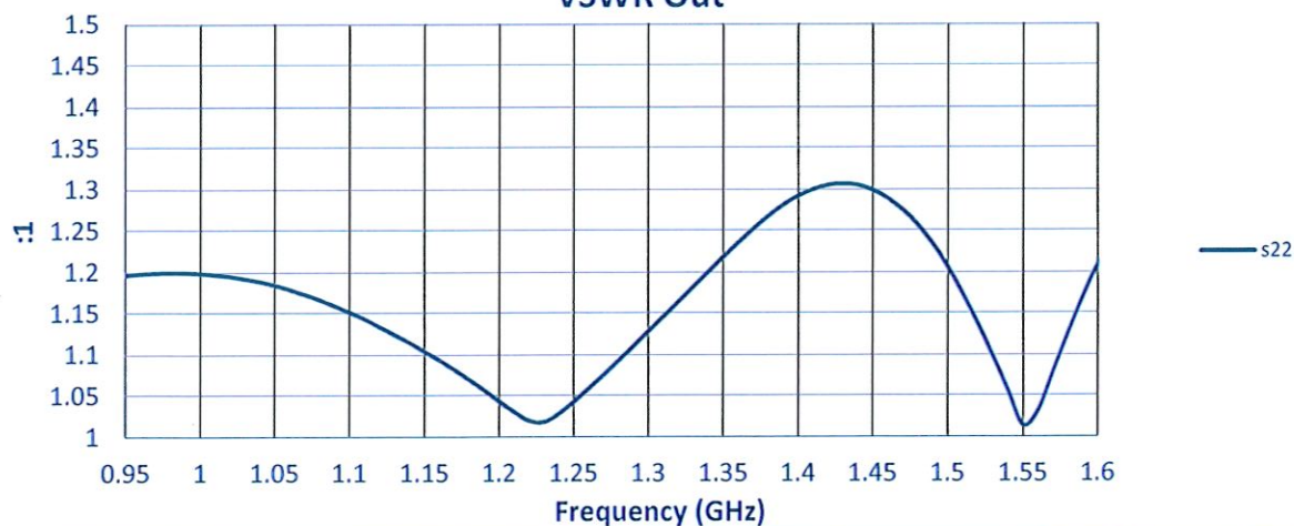
VSWR Out
