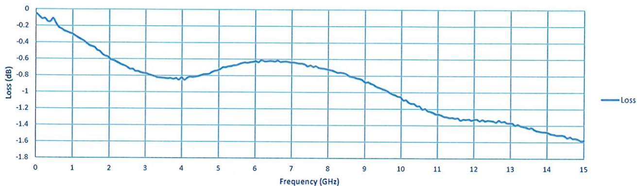
Insertion Loss
