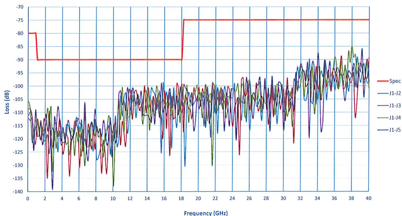
Isolation
