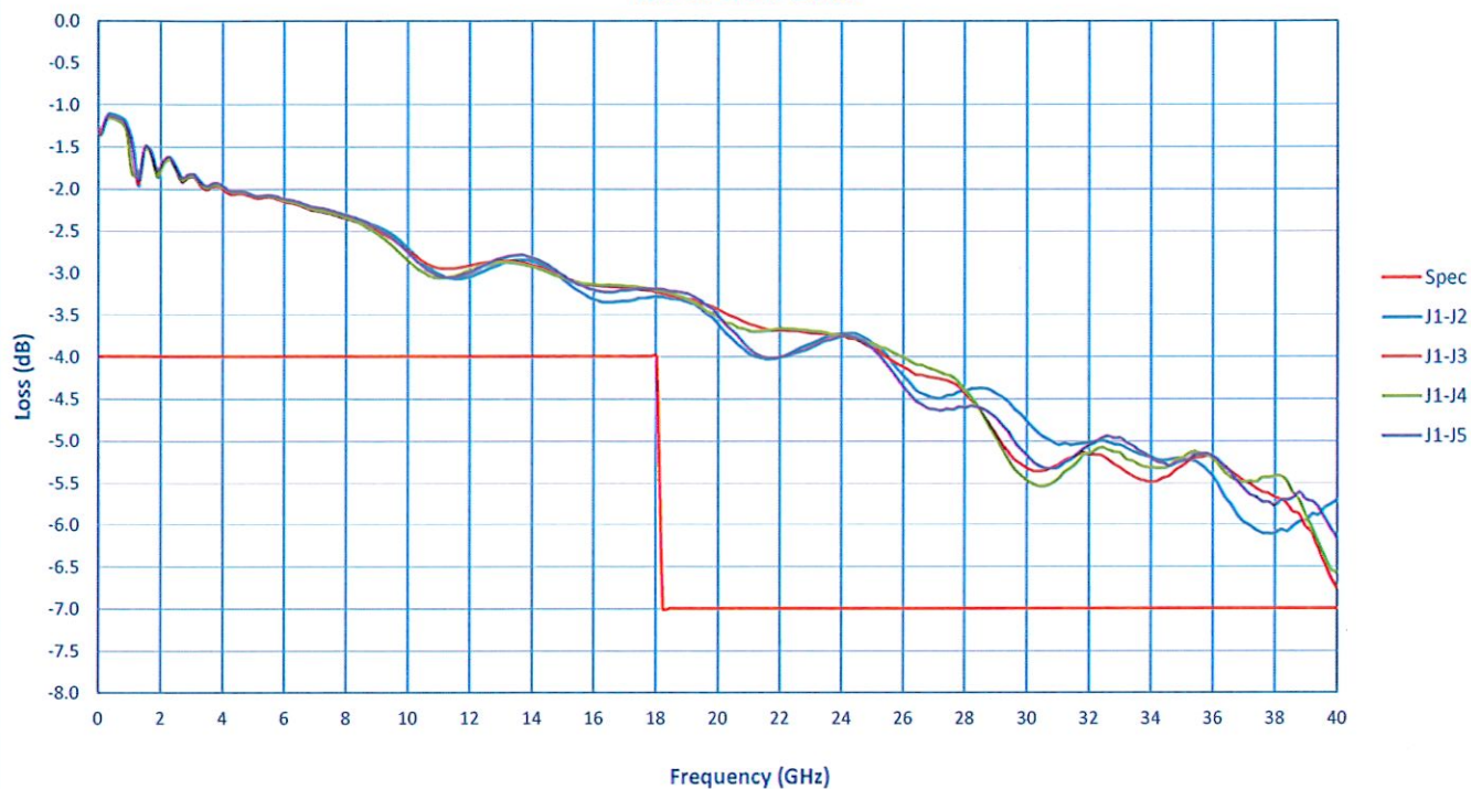
Insertion Loss
