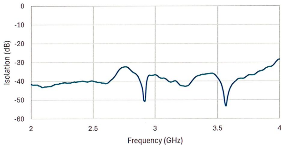
LO-IF Isolation
