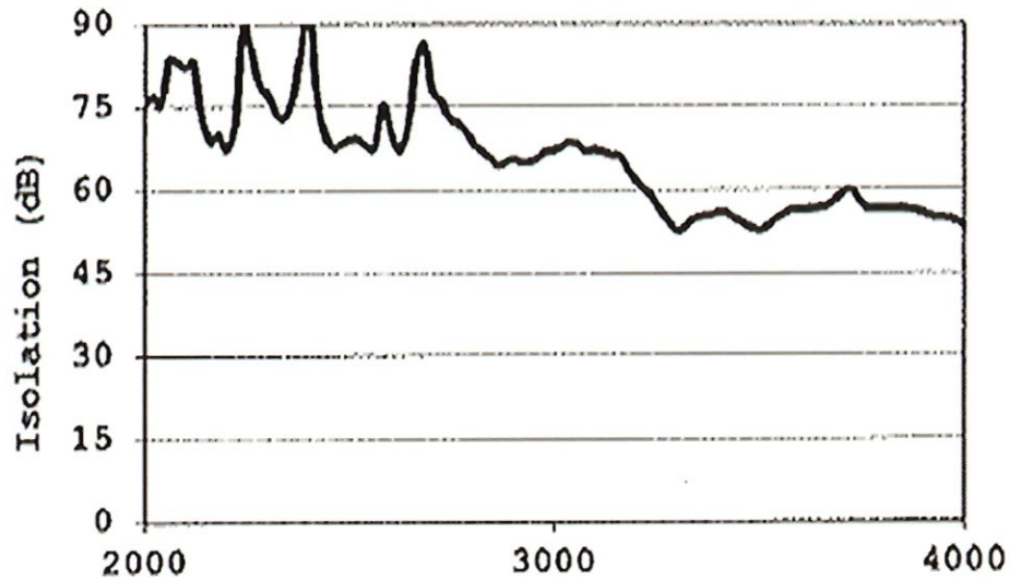
LO-RF ISOLATION
