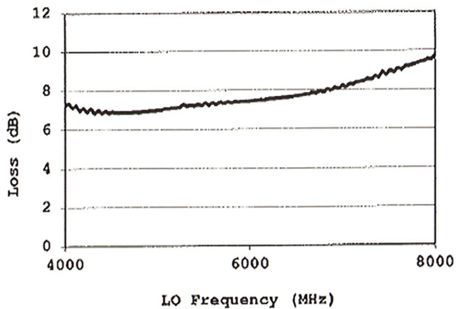
CONVERSION LOSS
