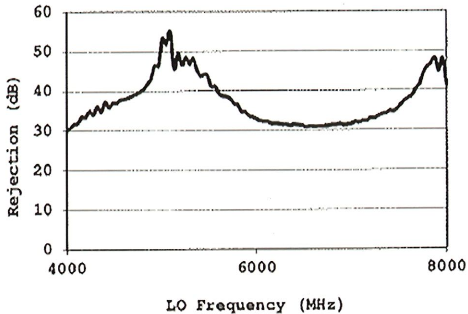
IMAGE REJECTION
