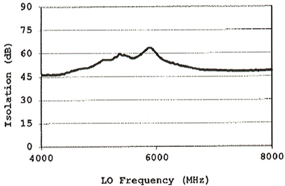
LO-RF ISOLATION
