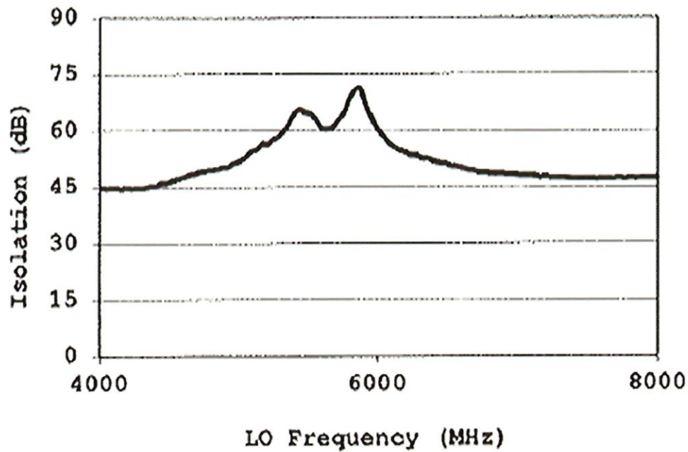
LO-RF ISOLATION
