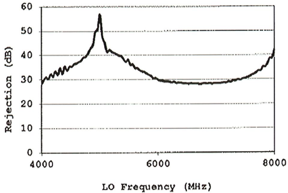
IMAGE REJECTION
