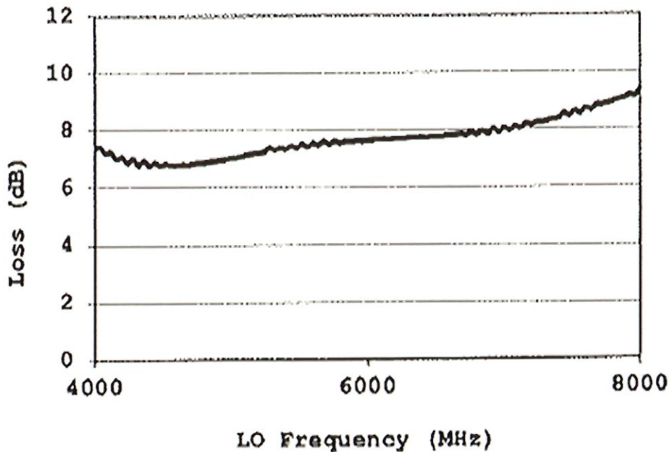
CONVERSION LOSS
