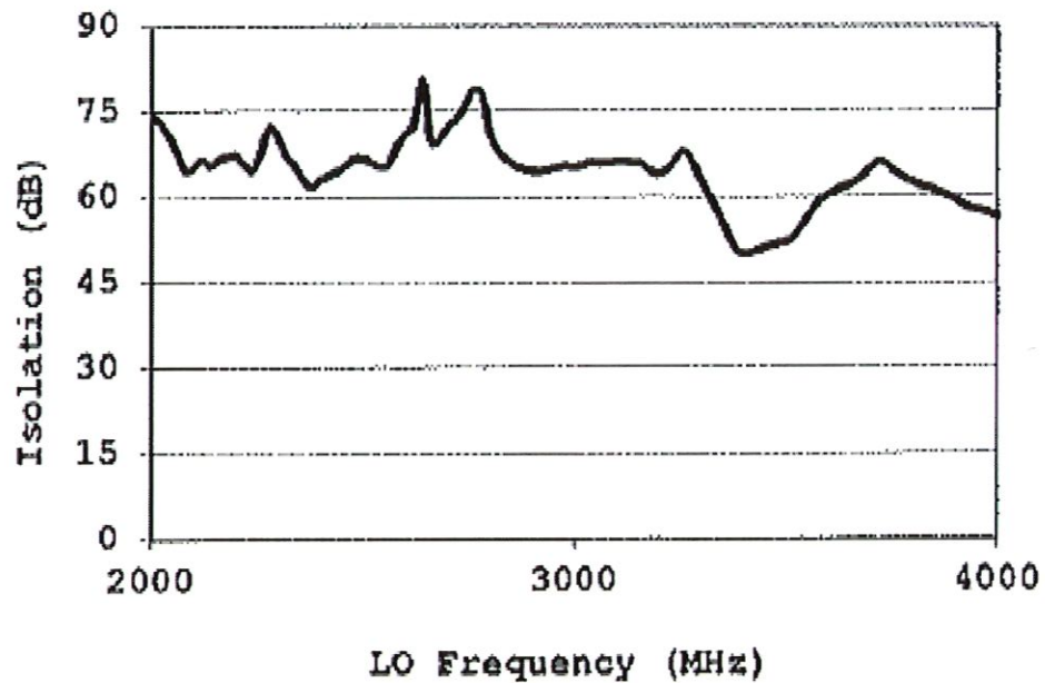
LO-RF ISOLATION
