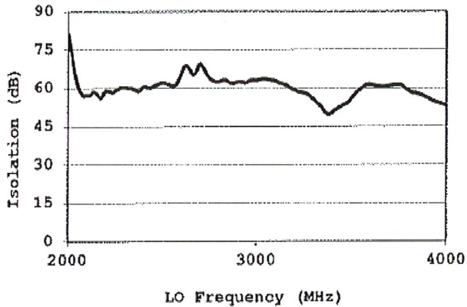
LO-RF ISOLATION
