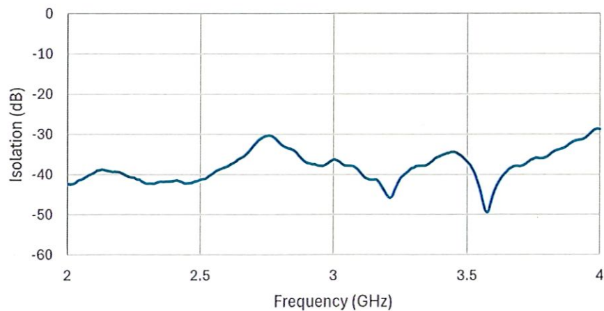
LO-IF Isolation
