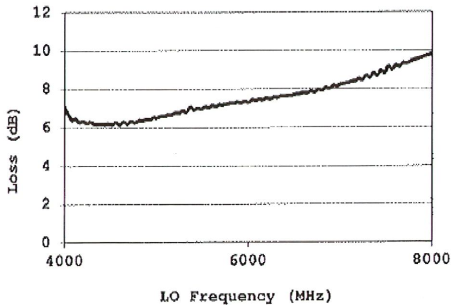
CONVERSION LOSS
