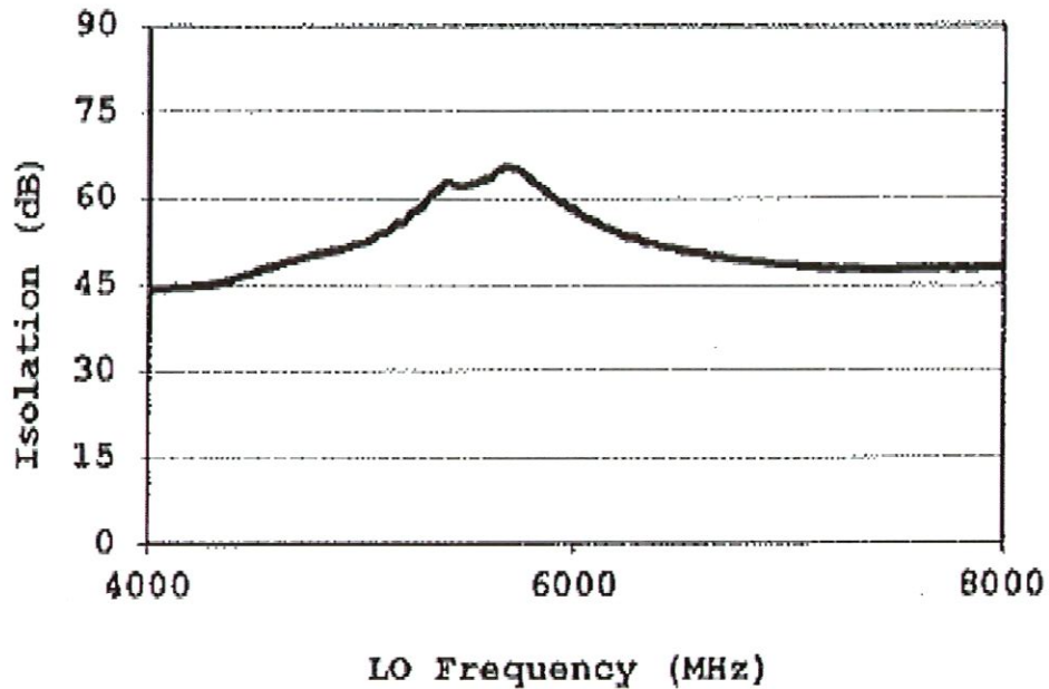
LO-RF ISOLATION
