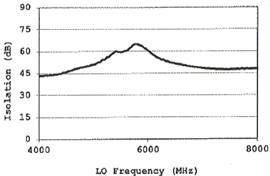
LO-RF ISOLATION
