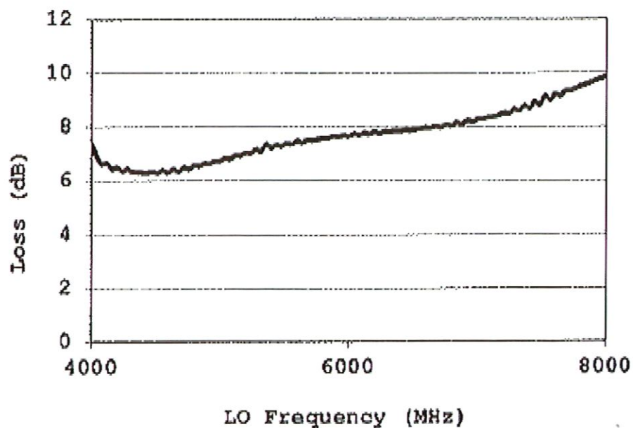
CONVERSION LOSS
