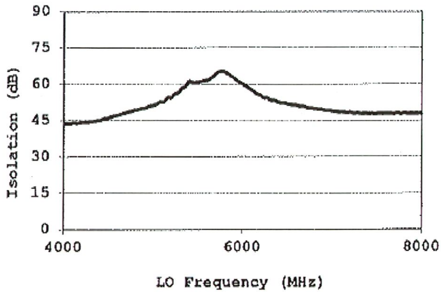
LO-RF ISOLATION
