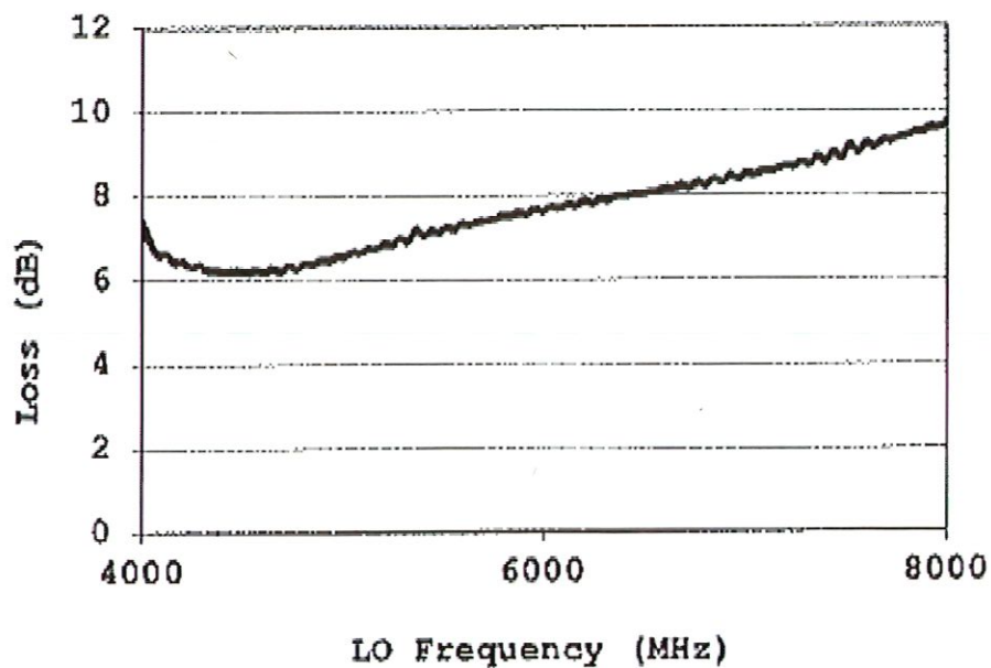
CONVERSION LOSS
