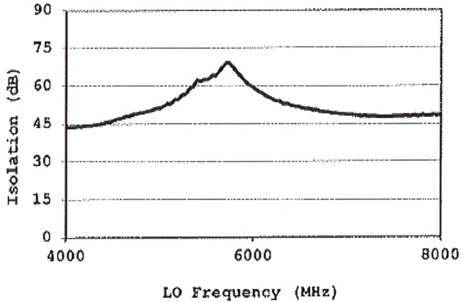
LO-RF ISOLATION
