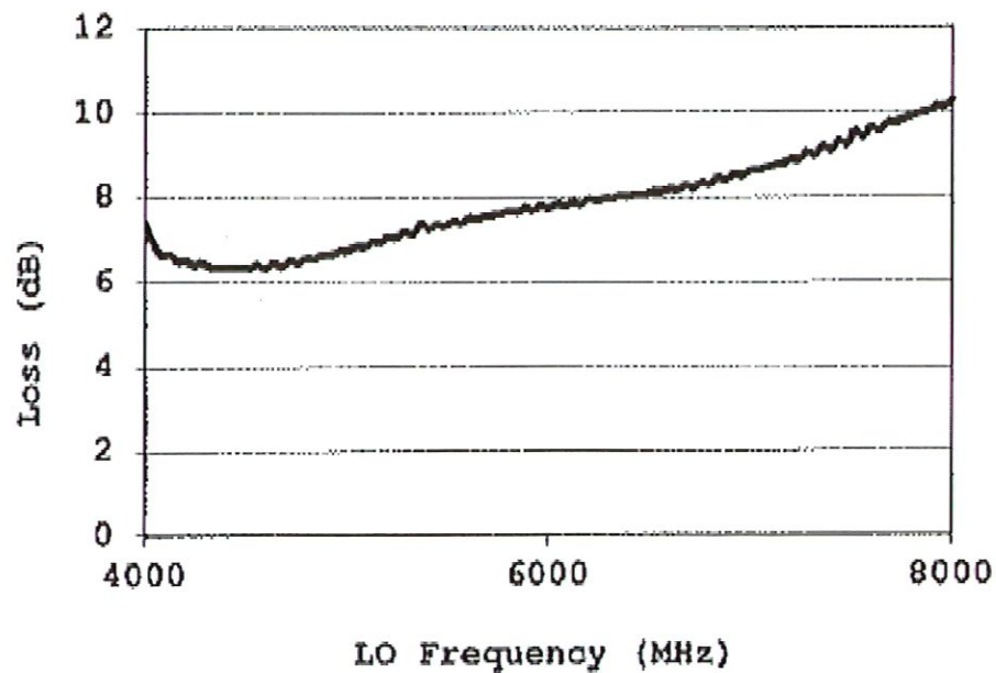
CONVERSION LOSS
