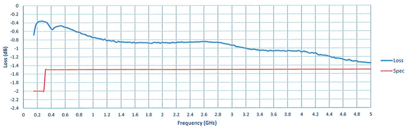
Insertion Loss
