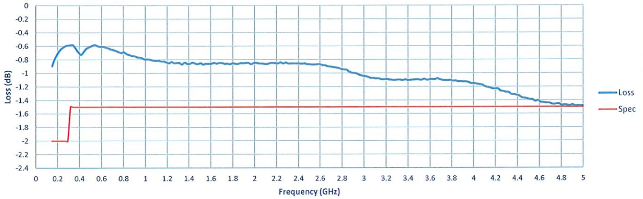
Insertion Loss
