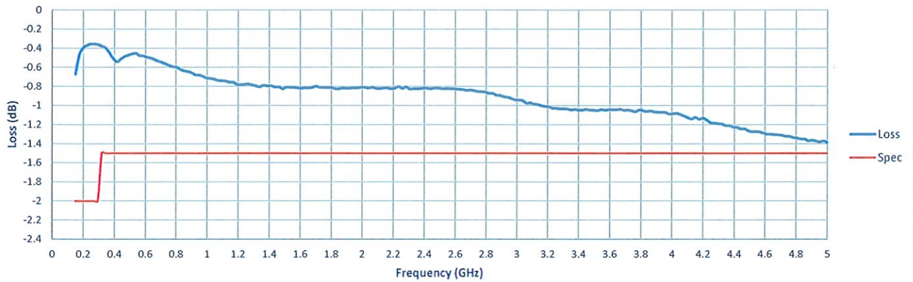
Insertion Loss
