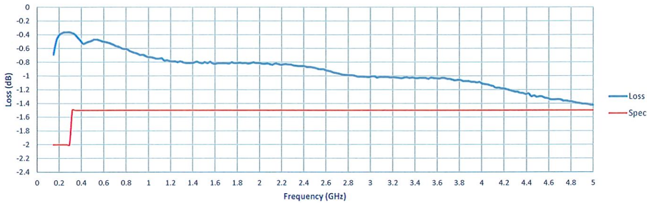
Insertion Loss
