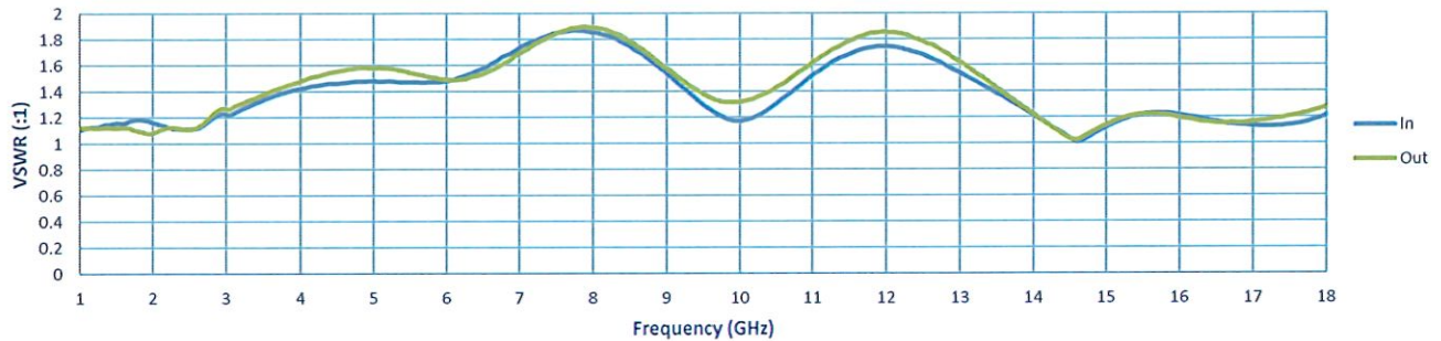
VSWR @ -20dBm
