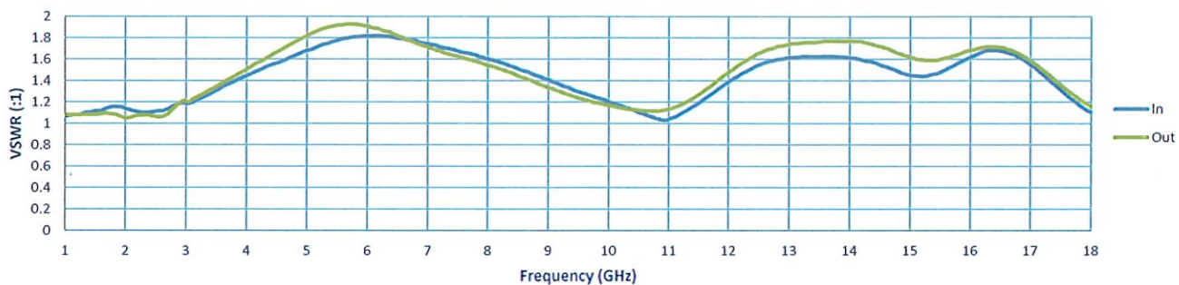
VSWR @ -20dBm
