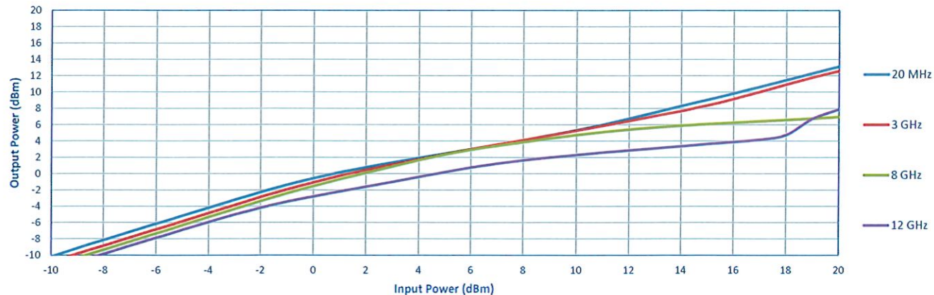
Limiting Curve
