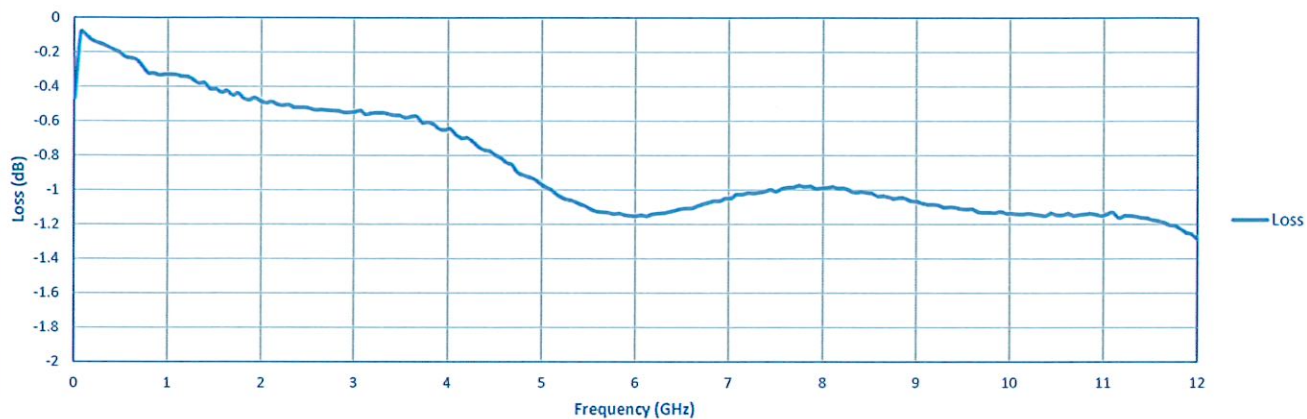
Insertion Loss
