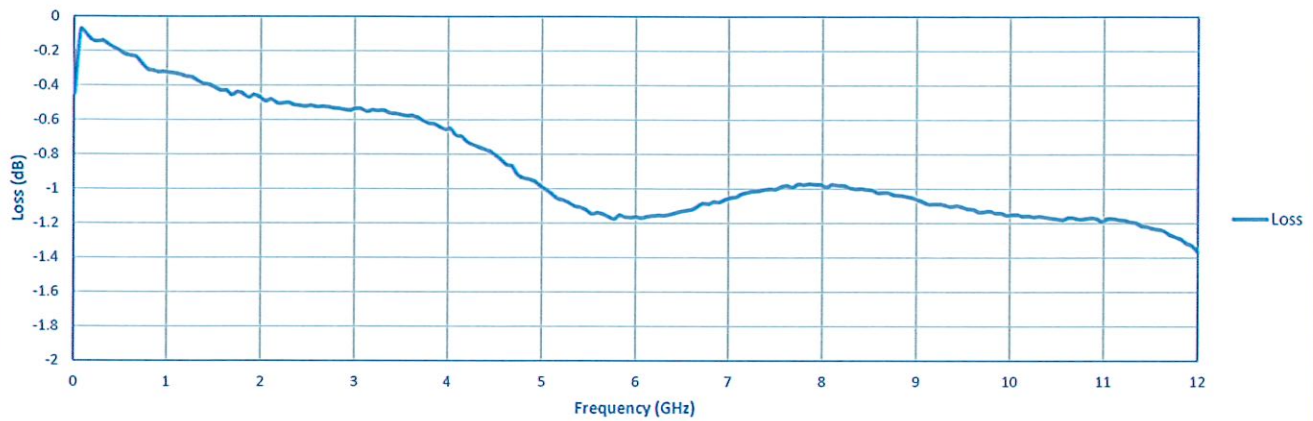
Insertion Loss
