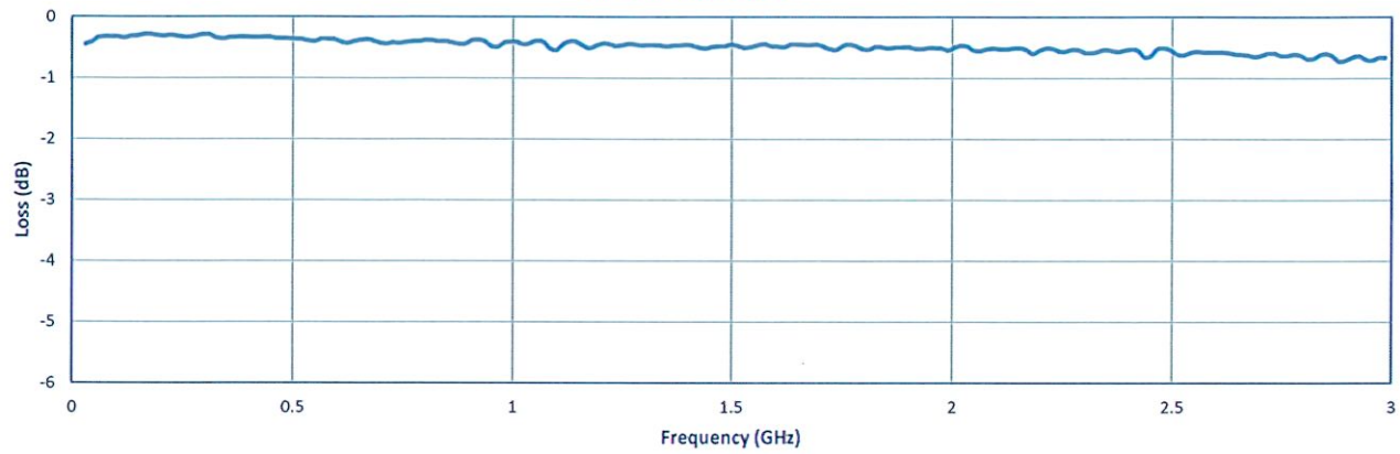
Insertion Loss
