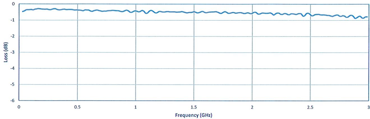
Insertion Loss
