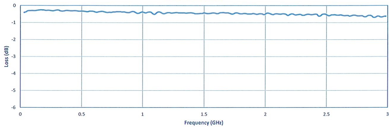
Insertion Loss
