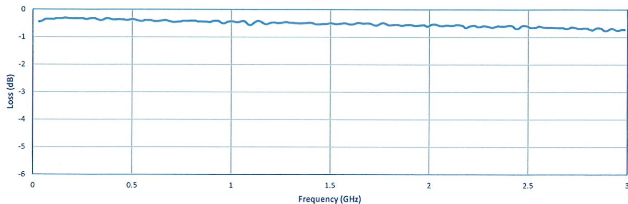
Insertion Loss
