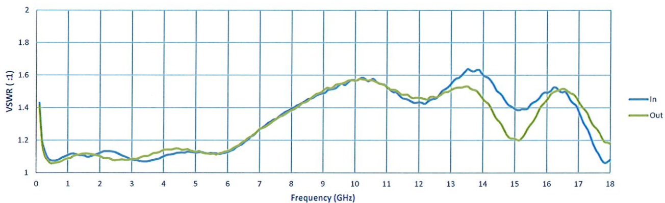
VSWR @ -20 dB
